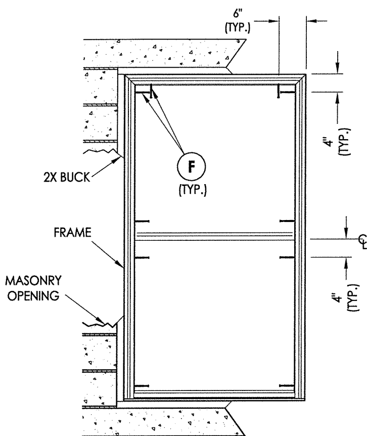
FRAME ANCHORING 2X BUCK
