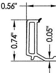
3 GLAZING BEAD
