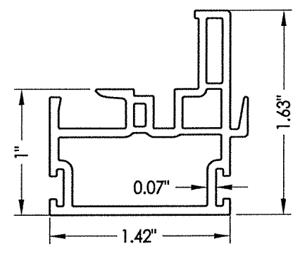
6 KEEPER RAIL
