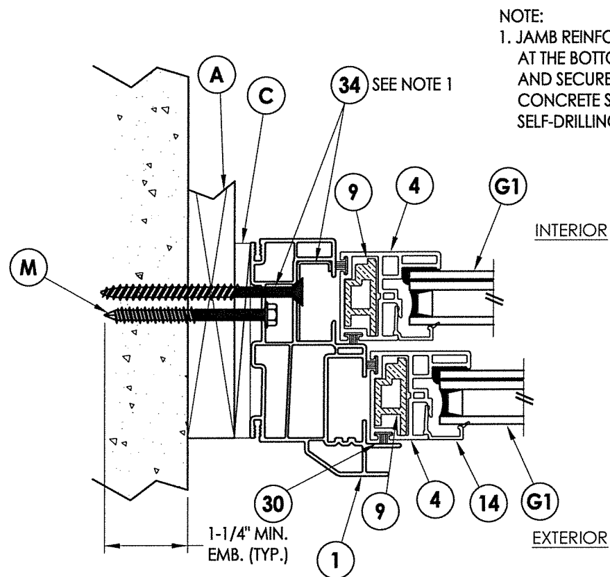
1 HORIZONTAL CROSS SECTION 3 Shown w/ 1X sub-buck
