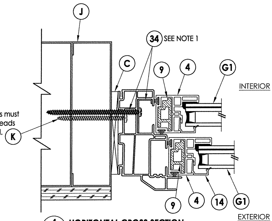
4 HORIZONTAL CROSS SECTION 3 Shown w/ Steel Stud Framing Option
