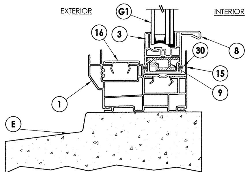
2 VERTICAL CROSS SECTION 3 Masonry sill
