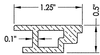
9 REINFORCEMENT (STILE)
