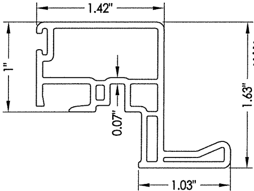
5 PULL RAIL
