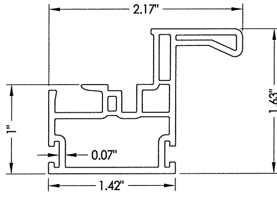
8 LIFT RAIL
