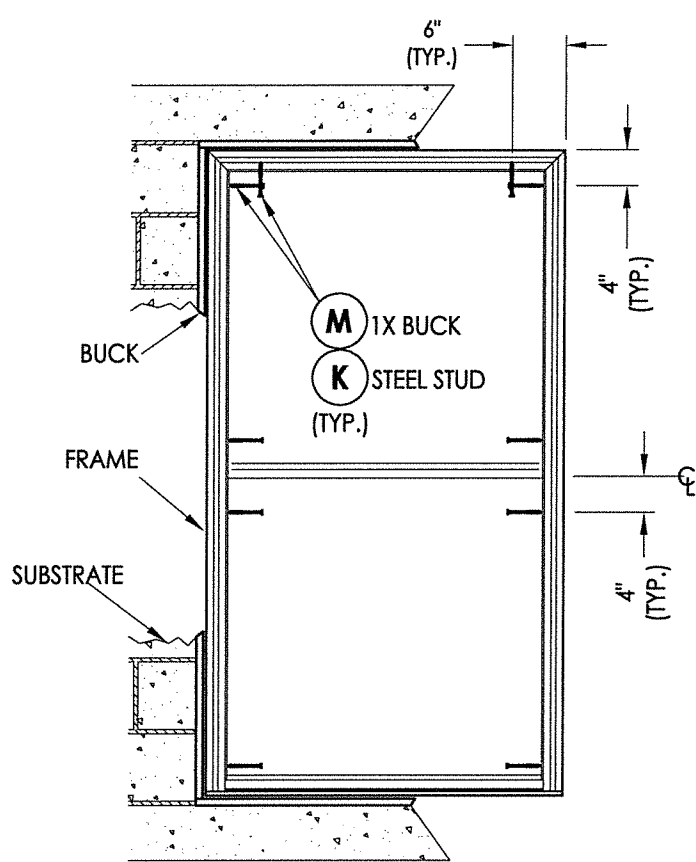
FRAME ANCHORING 1X BUCK/STEEL STUD
