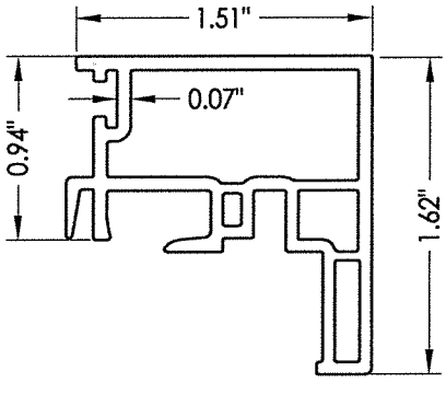
7 LOCK RAIL
