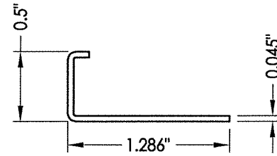
34 JAMB REINFORCEMENT CLIP 1" Wide
