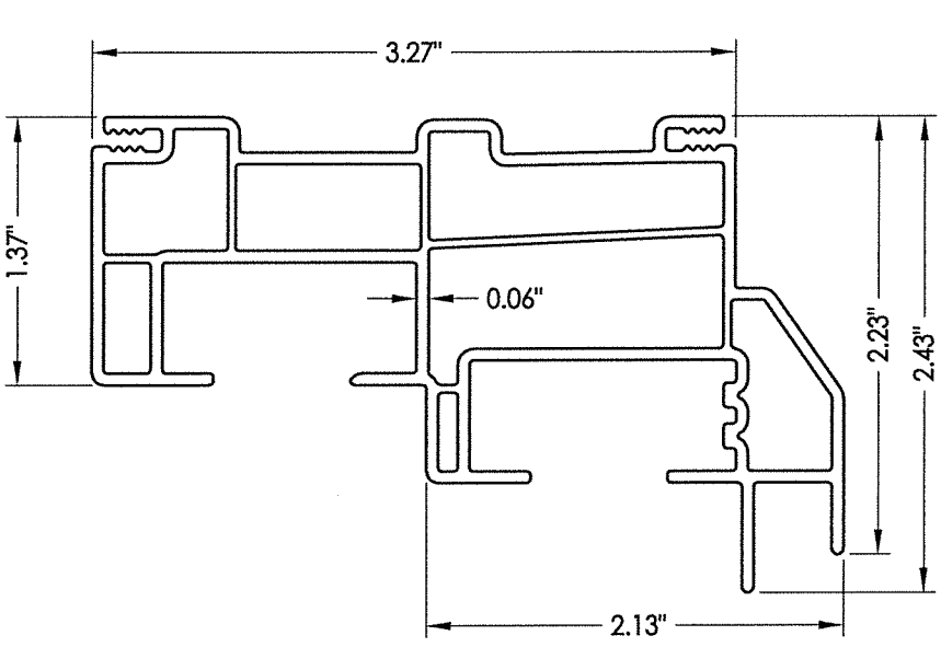
1 FRAME
