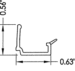
14 GLAZING BEAD
