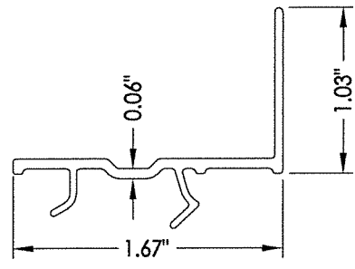
15 SILL ADAPTER
