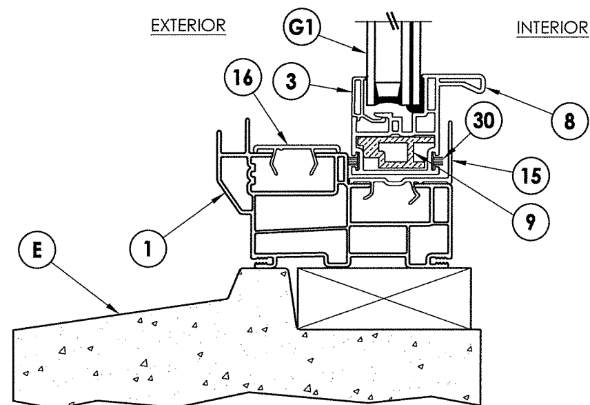
3 VERTICAL CROSS SECTION 3 Masonry sill
